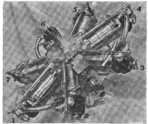
Timer and Exhaust Tappet Rods.
